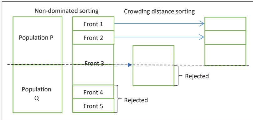
Flow Diagram of NSGA-II
